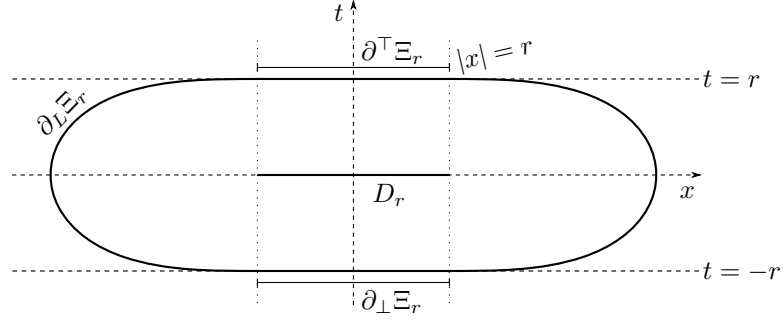
Figure 1: The boundary \partial \Xi_r of the set \Xi_r .
