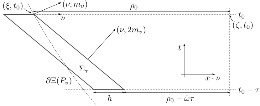
Figure 6: Construction of a test function \varphi in Lemma 3.21
