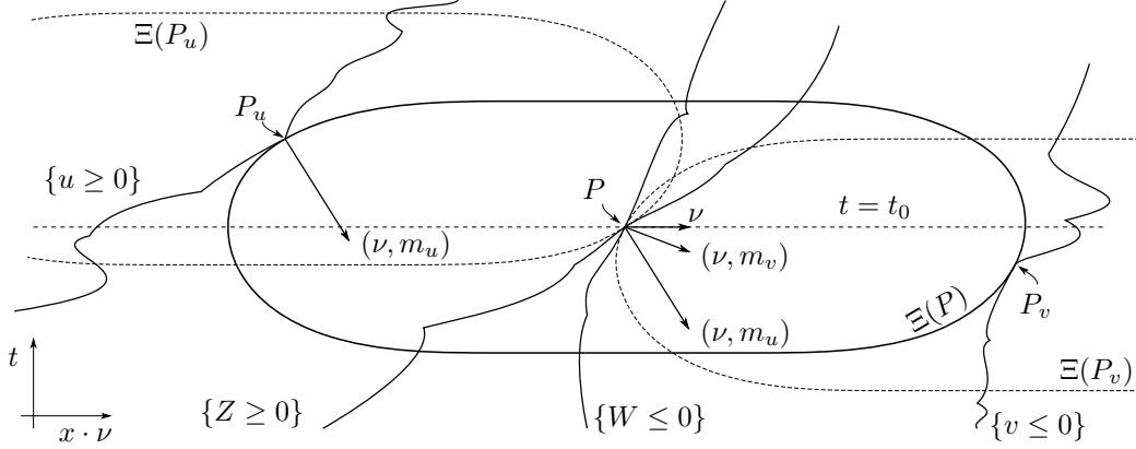
Figure 5: Situation at P = (\xi, t_0) \in \{Z \geq 0\} \cap \{W \leq 0\} .
