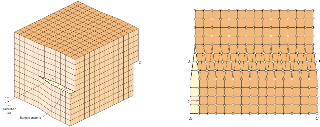
図 2: 螺旋転位. W. D. Callister, Jr., Materials science and engineering : an introduction, John Wiley & Sons, Inc., 1940, p. 90 (左), W. T. Read, Jr., Dislocations in Crystals, McGraw-Hill Book Company, New York, 1953 (右) より引用.
