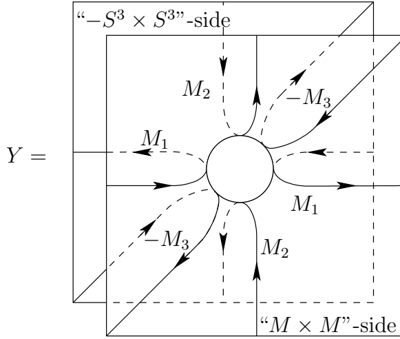
Fig. 1. The manifold pair (Y, Q) .
