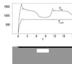
FIGURE 3. Controlled case: Temperature T_h in hot-spot of laser beam and T_{sub} close to lower end of desired hardening depth (top). Resulting austenite fraction (bottom).
