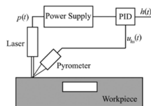
FIGURE 1. Pyrometer process control of laser surface hardening
