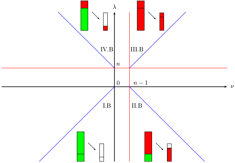
FIGURE 2.4. Image of \tilde{A}_{i,j} with (i, j) \in \mathcal{L}_{even}
