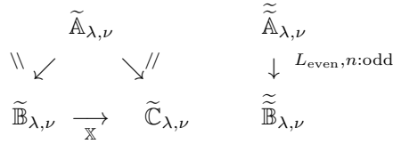
FIGURE 12.1. Reduction of operators
