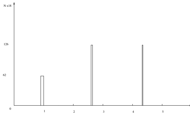
FIGURE 2. Mesoscopic profile of the rank \frac{3}{2} polyhedron of [6]
