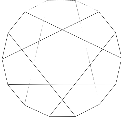
FIGURE 5. The incidence graph L_2 of the Fano plane and the link of X
