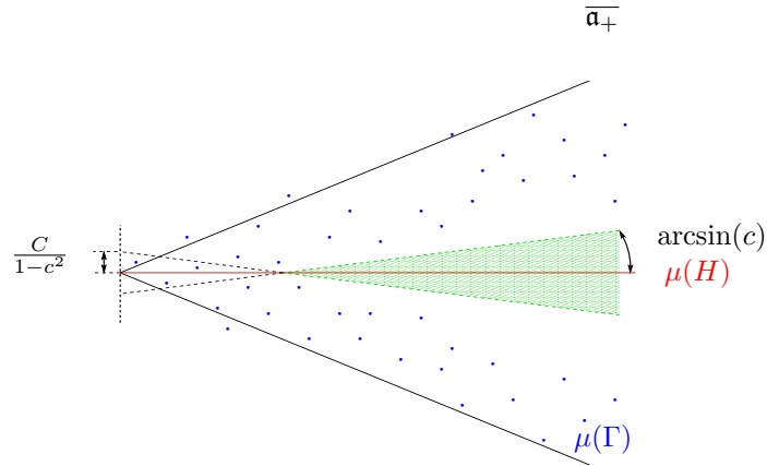
FIGURE 1. The Cartan projection of a (c, C) -sharp group \Gamma
